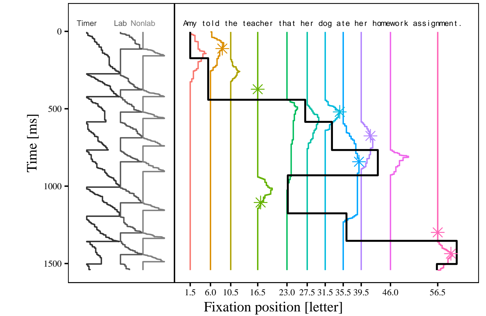
Figure 2. Simulated eye trajectory (solid black line) in the SWIFT model. Thin lines are word activations (colored) and timers (gray) as a function of time. Asterisks mark points in time when a saccade program is executed.
