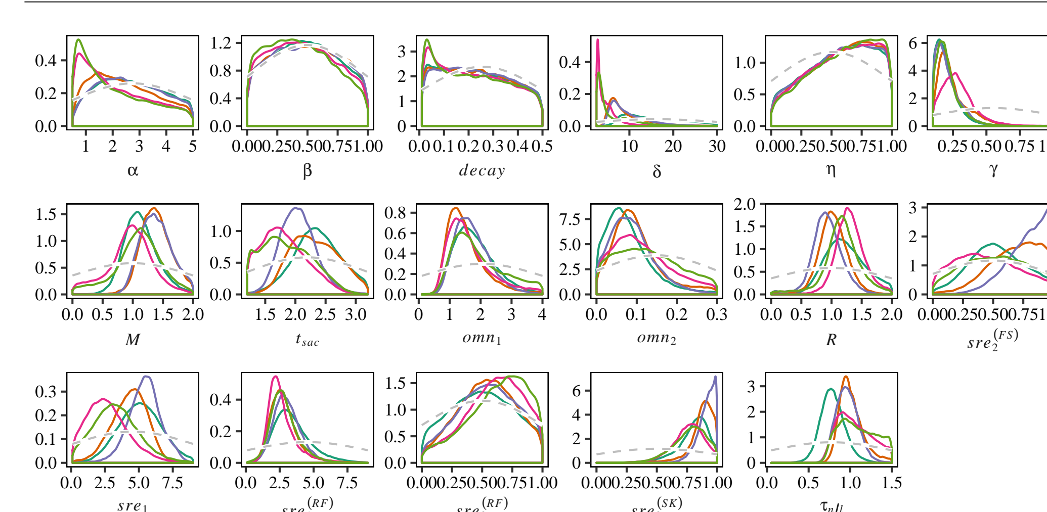
Figure 6. Posterior parameter distributions. Each color represents the aggregated sampled posteriors across all subjects in that condition. Priors (gray dashed lines) are truncated normal with support on 1 SD around the mean and were identical across subjects and conditions.
